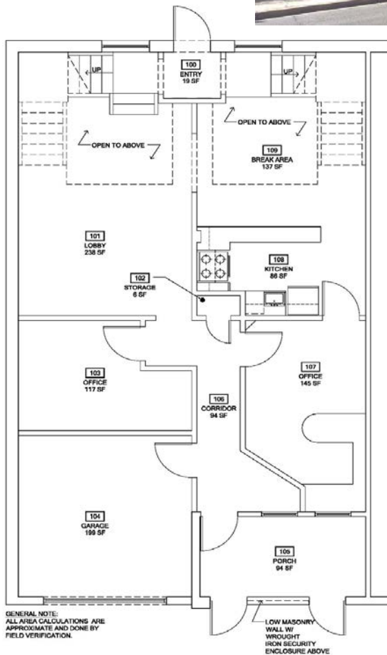
AS-BUILT - FIRST FLOOR PLAN 400 S. ERVAY ST. DALLAS TX 75206 DATE : 10.23.13 SCALE : 1/4" = 1'-0" WHEN PRINTED ON 11X17 PAPER
