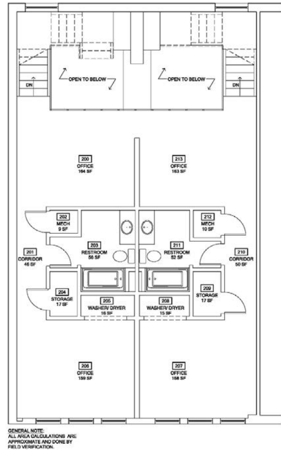
AS-BUILT - SECOND FLOOR PLAN 400 S. ERVAY ST. DALLAS TX 75206 DATE : 10.23.13 SCALE : 1/4" = 1'-0" WHEN PRINTED ON 11X17 PAPER
